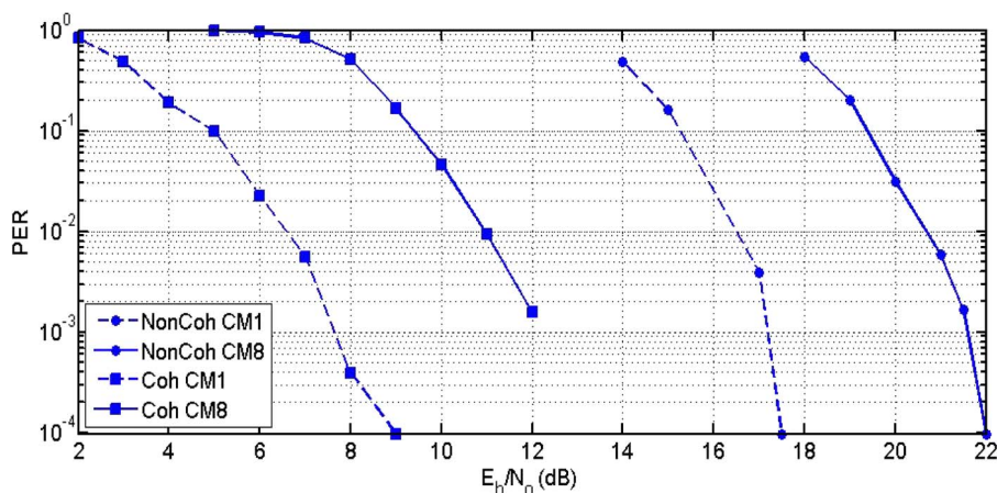
Fig. 11. Packet error rate versus E_b/N_o for coherent and noncoherent receivers over multipath channels.
