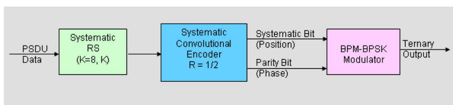
Fig. 9. IEEE 802.15.4a coding scheme for hybrid modulation.
